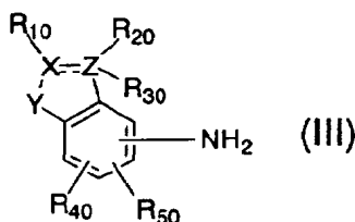
Formula (III)
